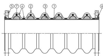
The shape of ZRJ-K400F
