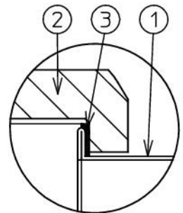
B部詳細 detail B
