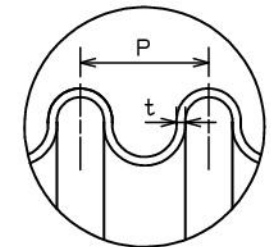
A部詳細 detail A
