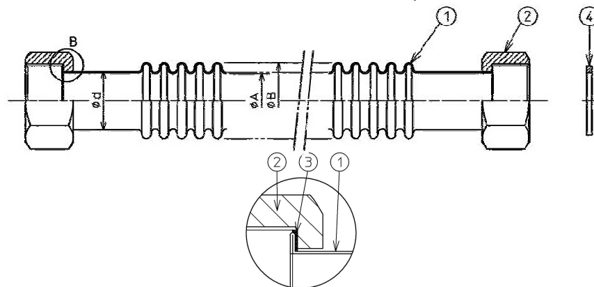
15A~32A Details B
